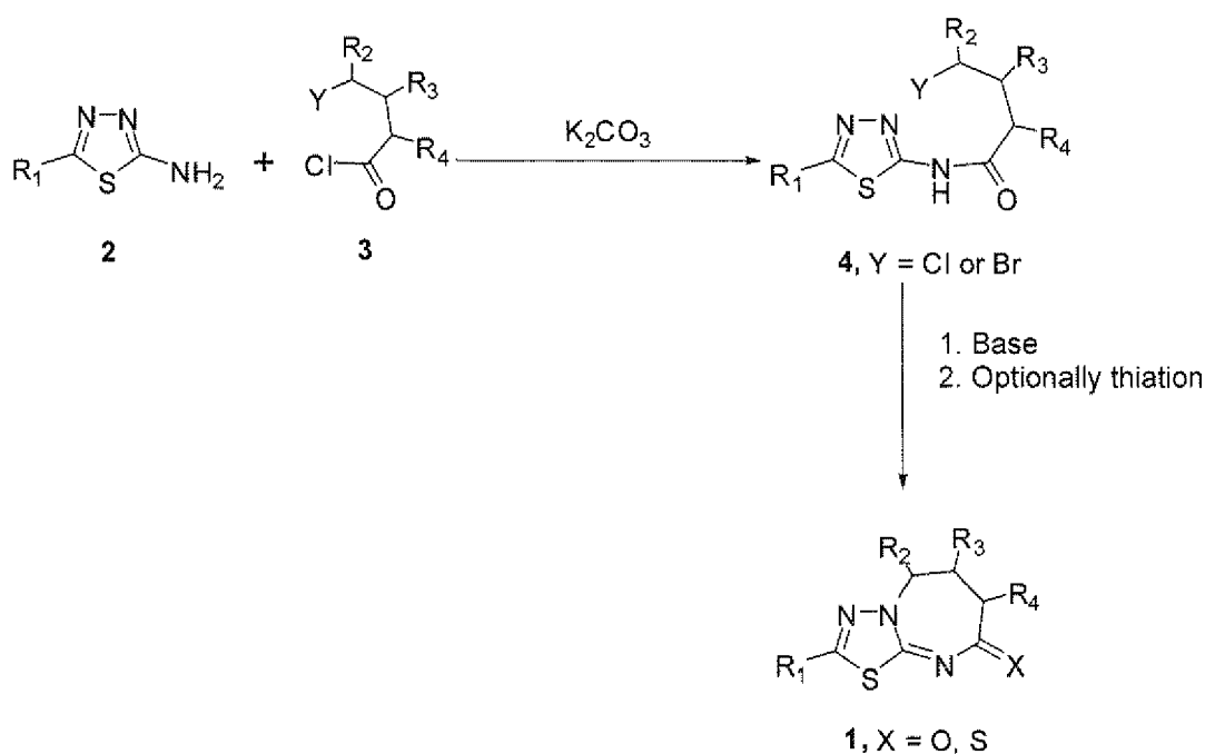
Scheme 1
